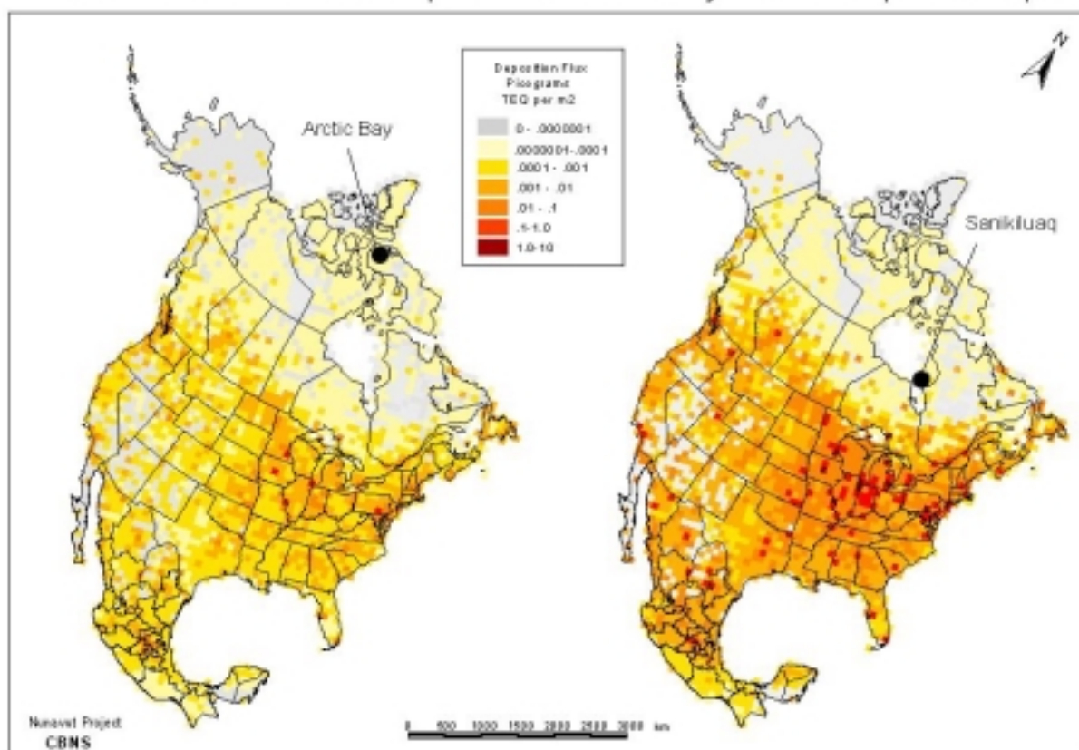
Figure 3.16 Dioxin Source Contributions to Deposition Flux at Arctic Bay and Sanikiluaq Land Receptors
