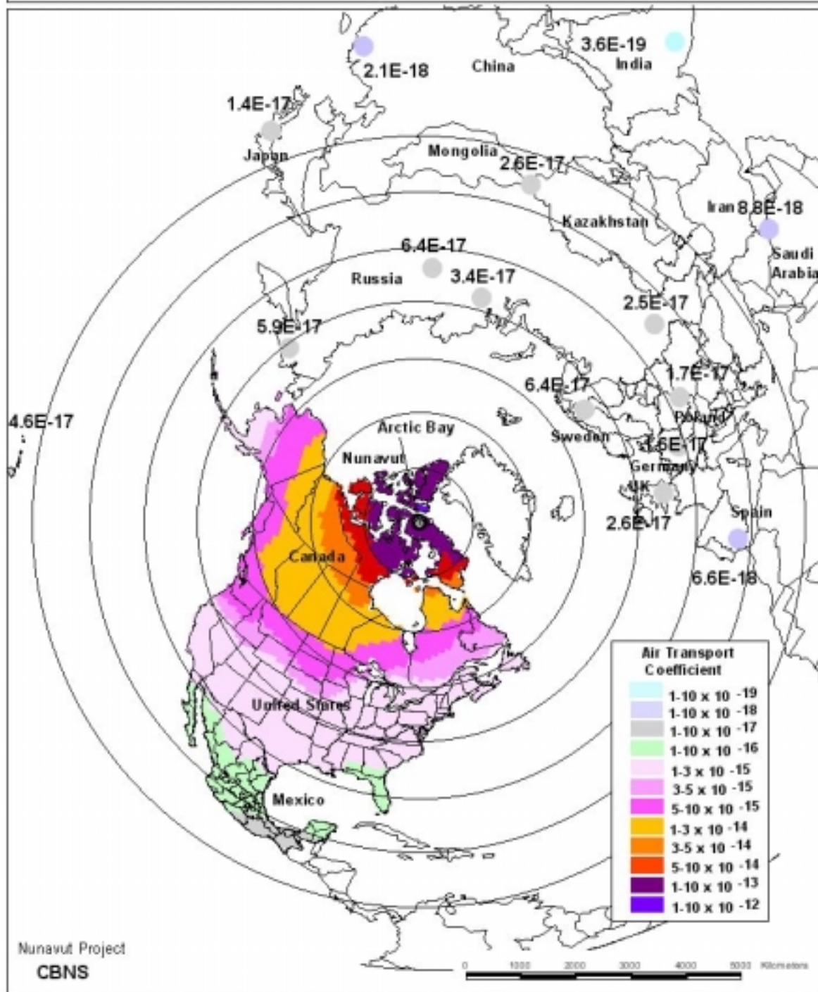
Figure 3.18 Annual OCDD Deposition Air Transport Coefficients from Standard (Hypothetical) Source Points in Europe and Asia to Arctic Bay, Marine Receptor
