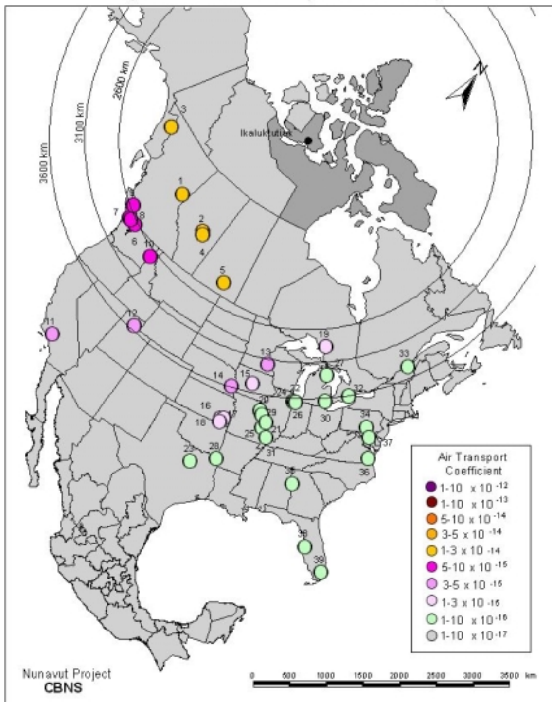
Figure 3.7C Air Transport Coefficients of the Highest-Ranked Sources (39) Contributing to 35% of the Total Deposition at Ikaluktutiak Land Receptor. (Numbers indicate Air Transport Coefficient rank)
