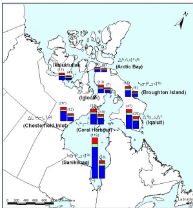
Figure 3.1 Dioxin Deposition at Nunavut Receptors
