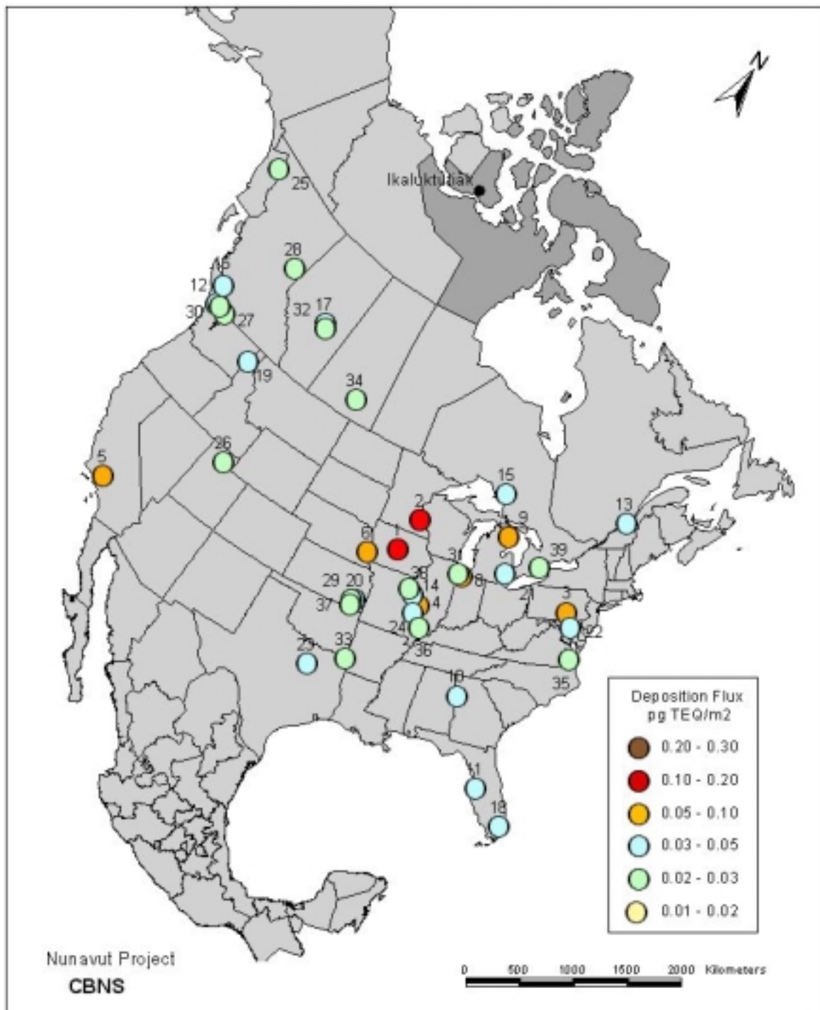
Figure 3.7B Dioxin Deposition Due to the Highest-Ranked Sources (39) Contributing to 35% of the Total Dioxin Deposition at Ikaluktutiak Land Receptor. (Numbers show deposition rank)
