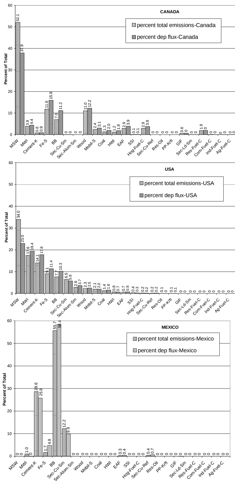
Fig. 3.3 DIOXIN SOURCE CLASS PERCENT OF EMISSIONS DEPOSITION FLUX
