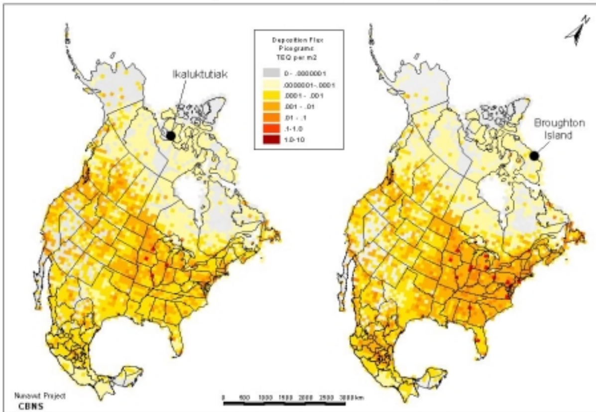
Figure 3.17 Dioxin Source Contributions to Deposition Flux at Ikaluktutiak and Broughton Island Land Receptor
