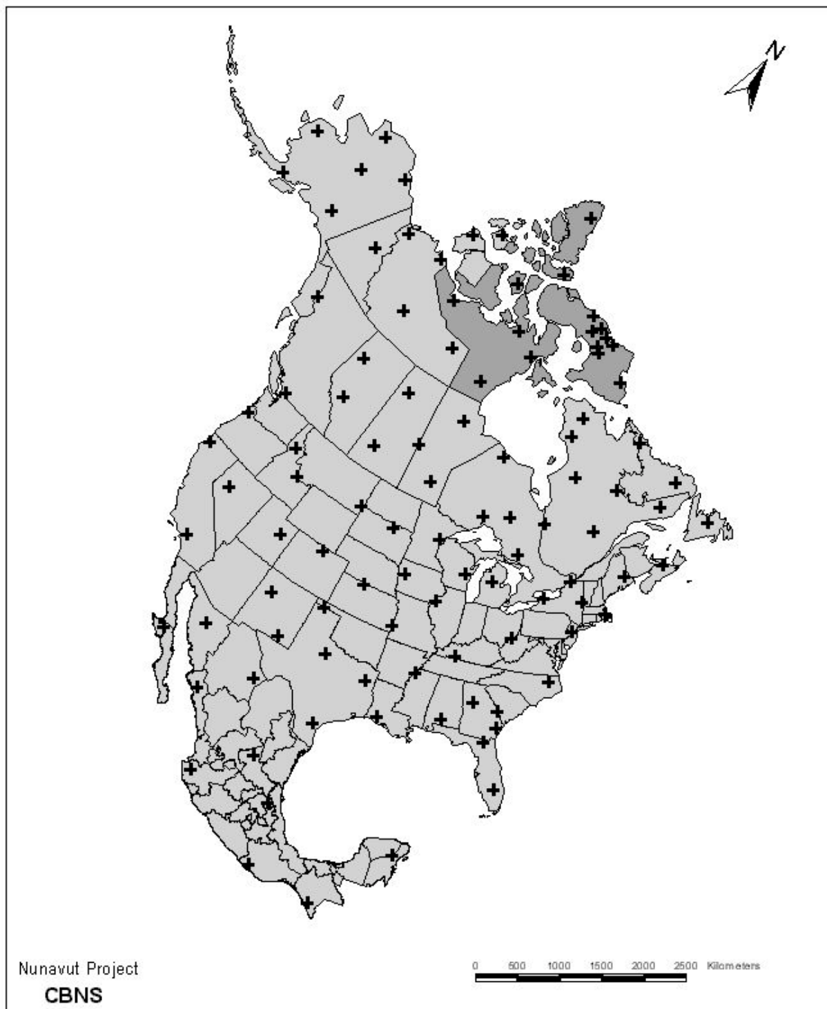
FIG. 2.2 STANDARD (HYPOTHETICAL) SOURCE POINTS
