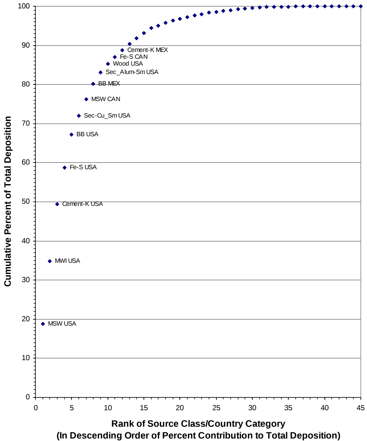
Figure 3.5 Cumulative Contributions of the 45 Source Class/Country Categories to Dioxin Deposition at Coral Harbour ( n9oĴ ) Land Receptor
