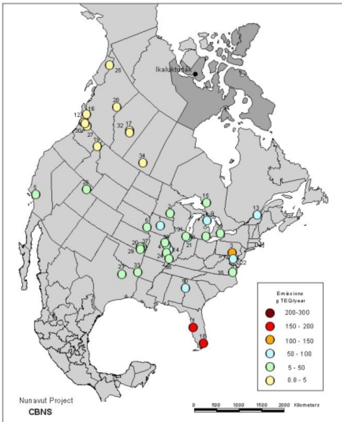
Figure 3.7A Dioxin Emissions Due to the Highest-Ranked Sources (39) Contributing to 35% of the Total Dioxin Deposition at Ikaluktutiak Land Receptor.
