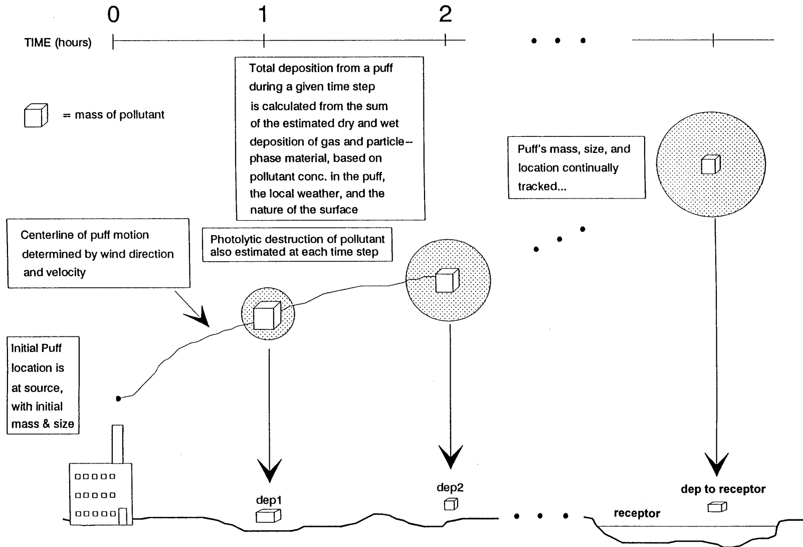
Figure 2.1 HYSPLIT Air Transport and Deposition Model
