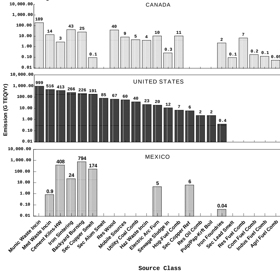
Figure 2.6: The North American Dioxin Source Emission Inventories
