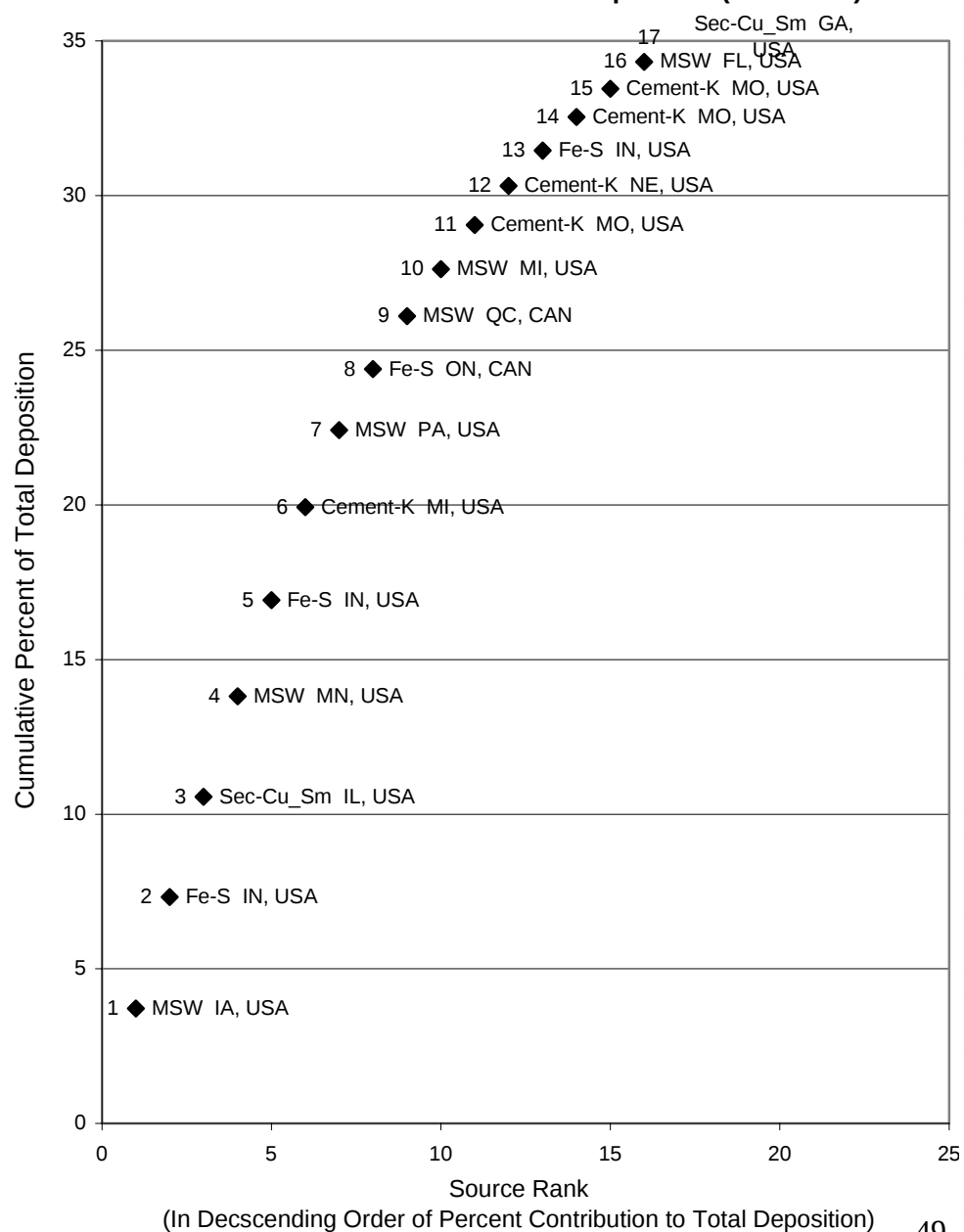
Figure 3.6H Sanikiluaq Land Receptor
