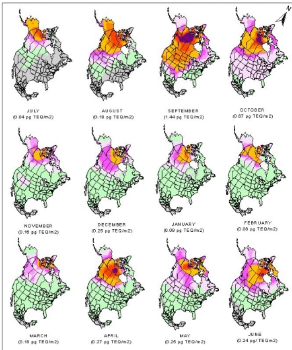
Figure 3.15 A Monthly Dioxin AirTransport Coefficients & Deposition Flux (pg TEQ/m 2 ) to Ikaluktutiak Land Receptor (July 1996-June 1997)
