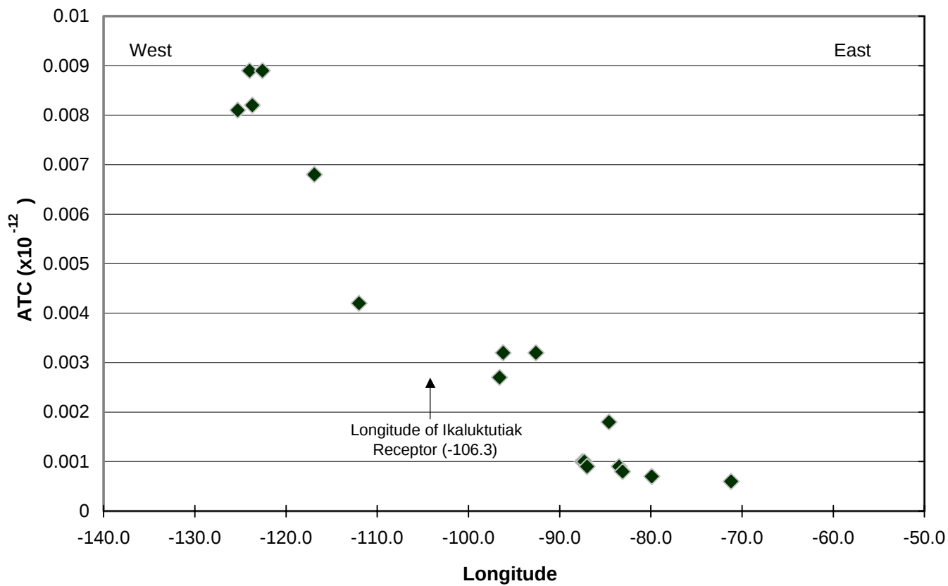
Figure 3.8 Relation Between Air Transport Coefficient (ATC) and Longitude for Highest Sources that Contribute to 35% of Dioxin Deposition at Ikaluktutiak Land Receptor and are Aproximately Equidistant (3100±500 km) from Receptor
