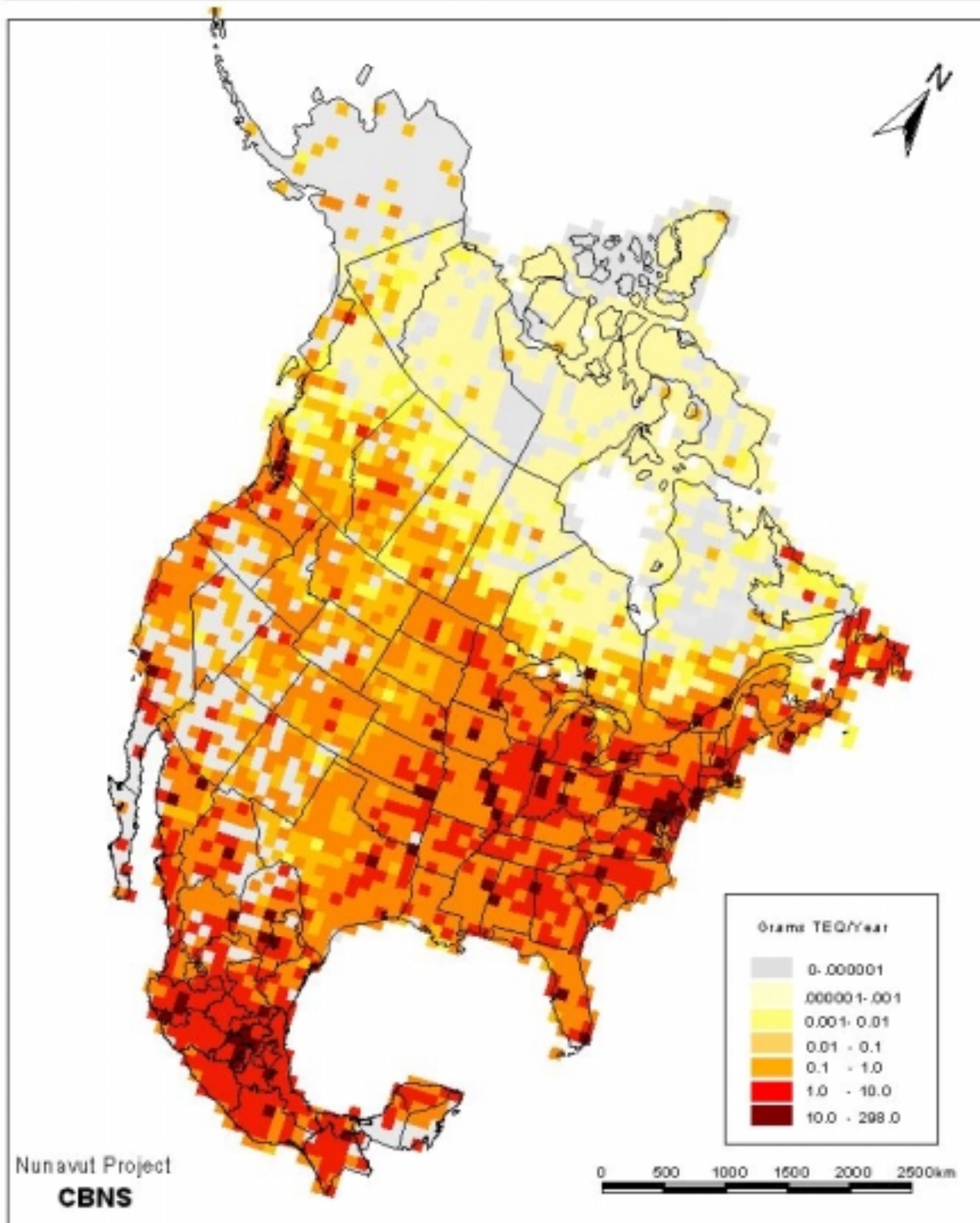
Figure 3.9 Geographic Distribution of Annual Dioxin Emission from North American Sources, 1996-1997
