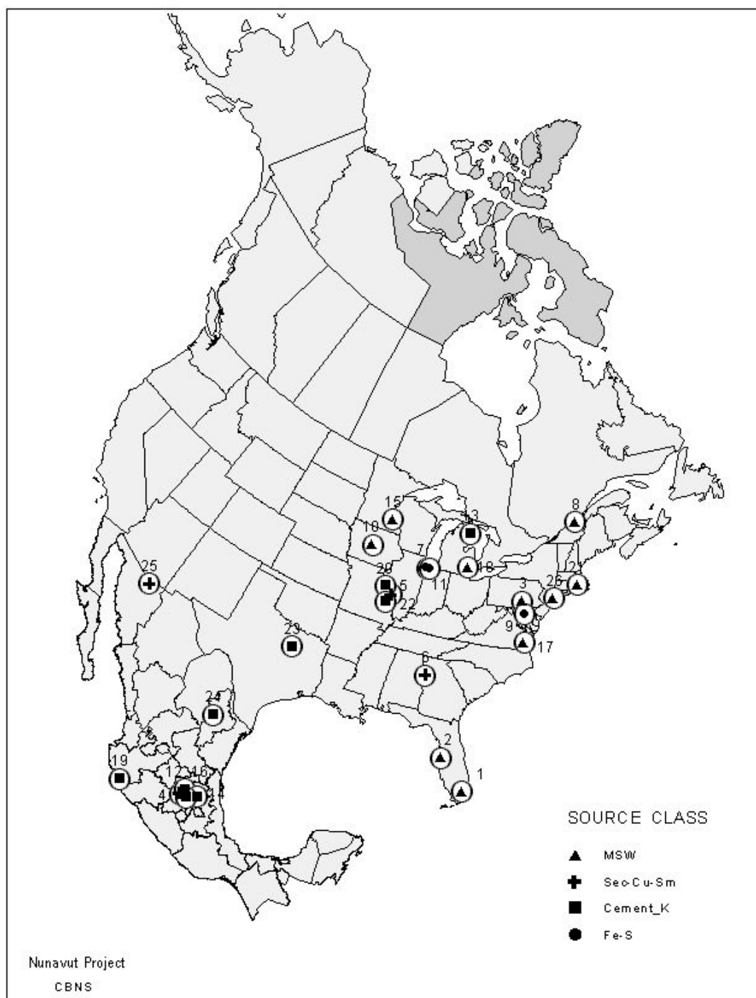
Figure 3.10 Highest-Ranked Individual Sources that Account for 35% of Total Dioxin Emissions
