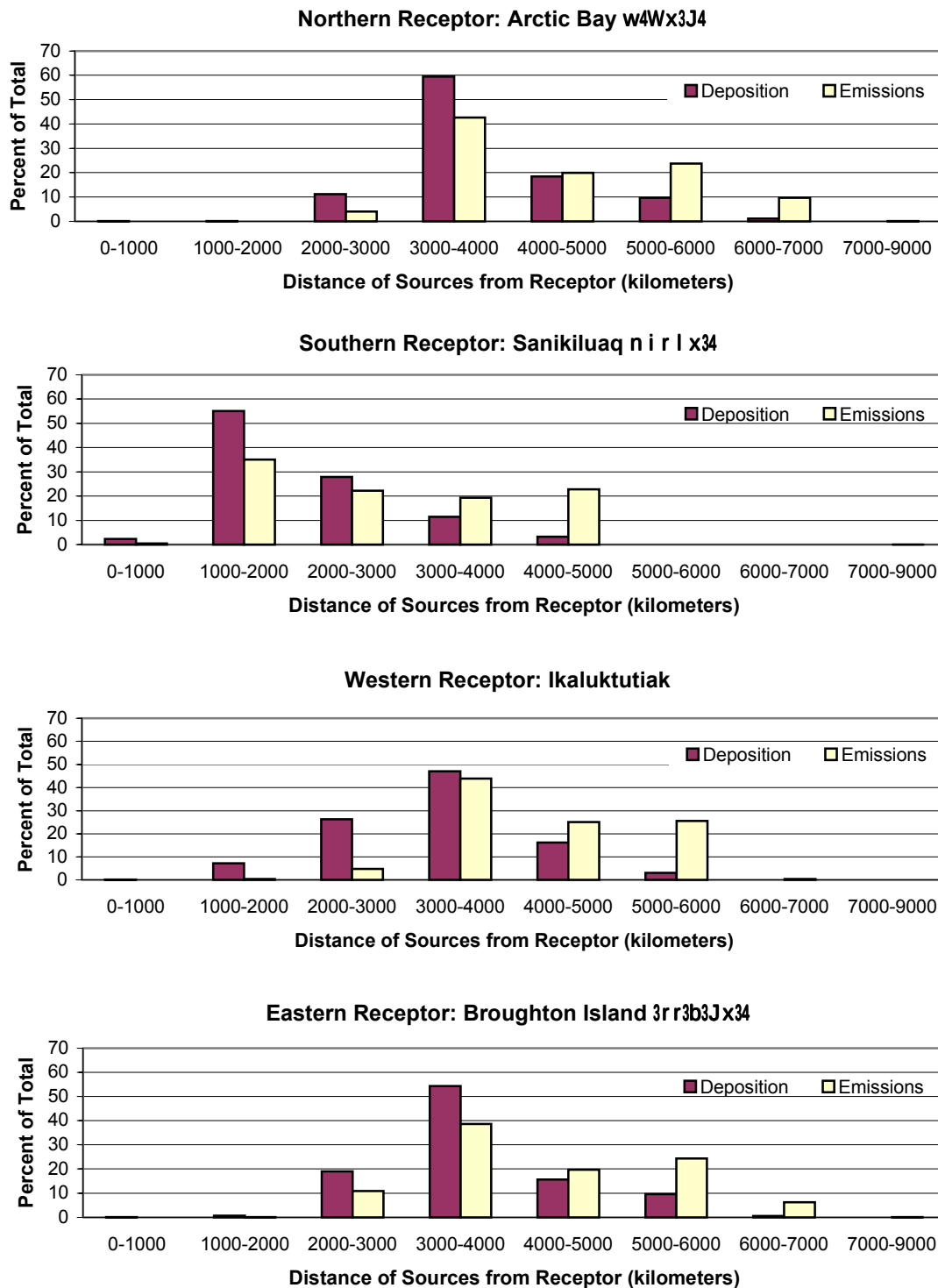
Figure 3.4 Dioxin Emissions and Deposition as a Function of the Distance of Sources from Selected Nunavut Land Receptors
